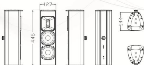
CL4023B/CL4023W
