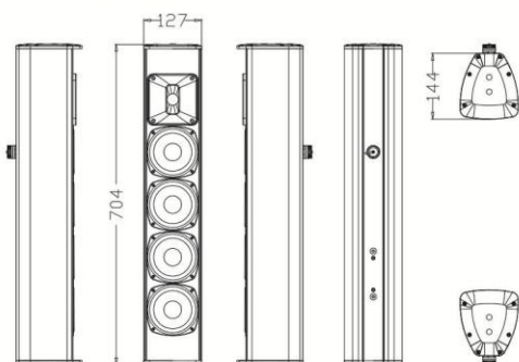
CL4025B/CL4025W
